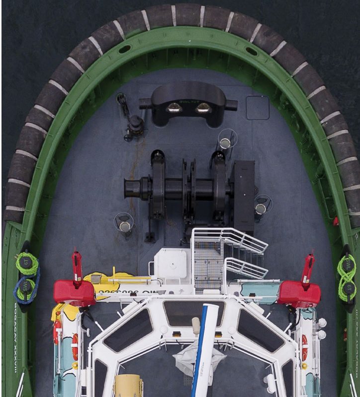
Electric Towing Winch delivered to equip a 60T Mtug
